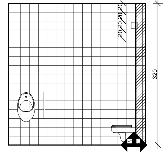
RŚ-01/04
