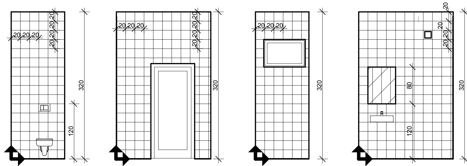
RŚ-06/01 1:50 RŚ-06/02 1:50 RŚ-06/03 1:50 RŚ-06/04 1:50
