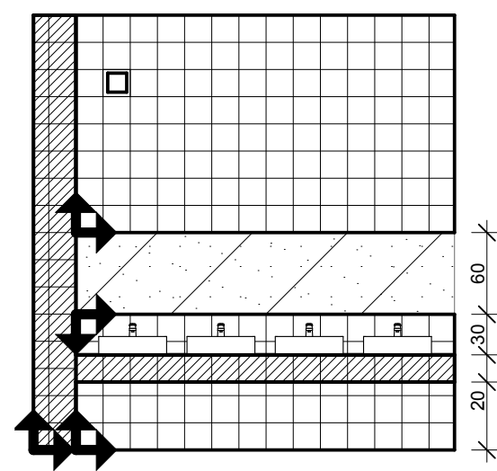
RŚ-03/02 1:50
