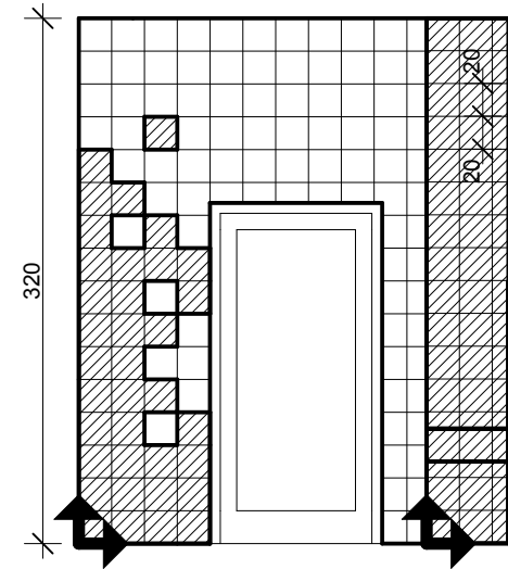
RŚ-03/01 1:50
