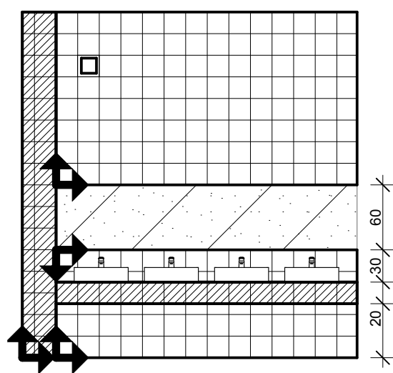
RŚ-03/02
