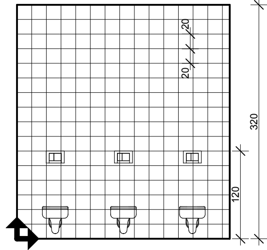
RŚ-02/01
